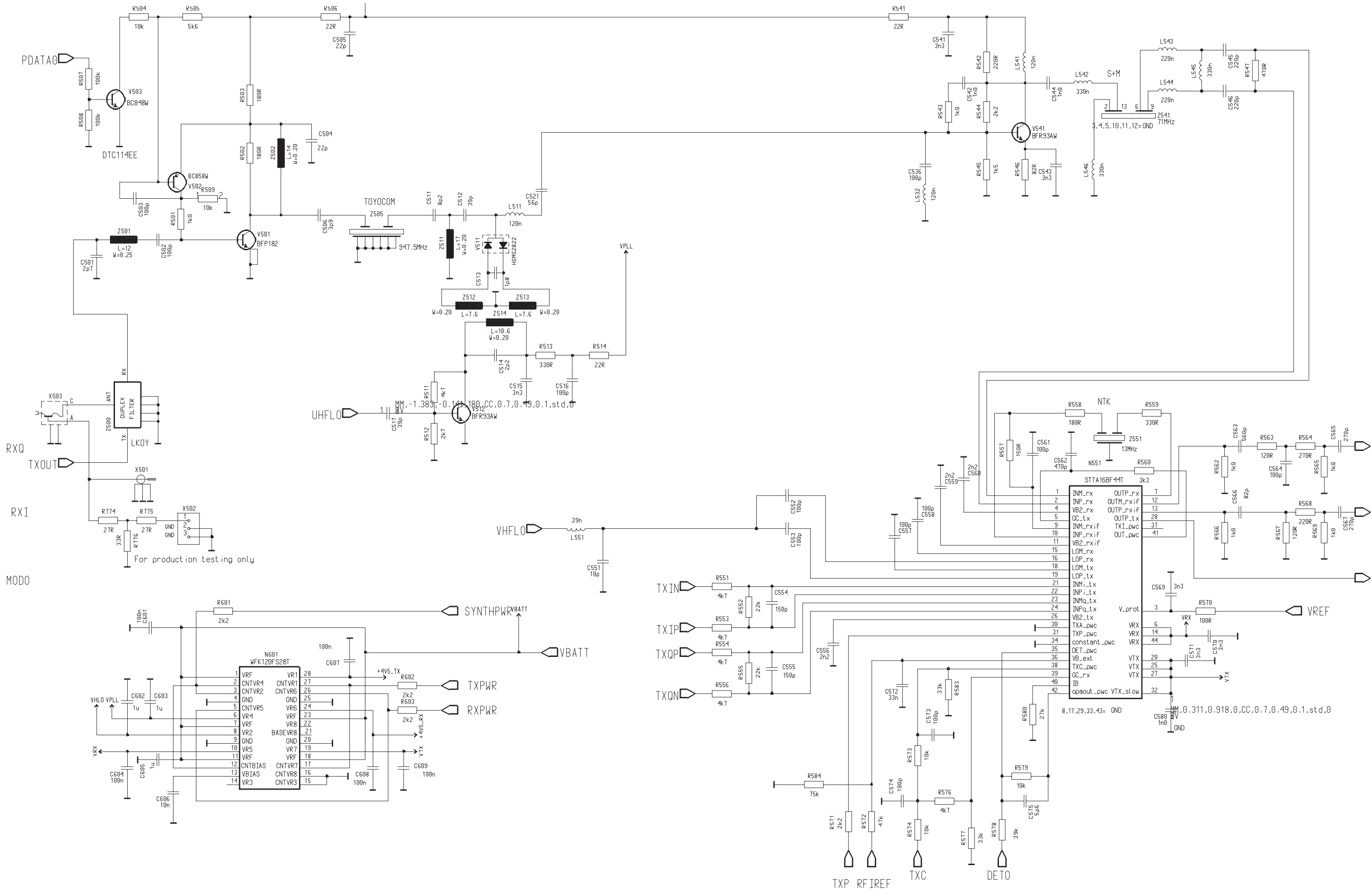
Figure 7 RF / RX Circuit Diagram
